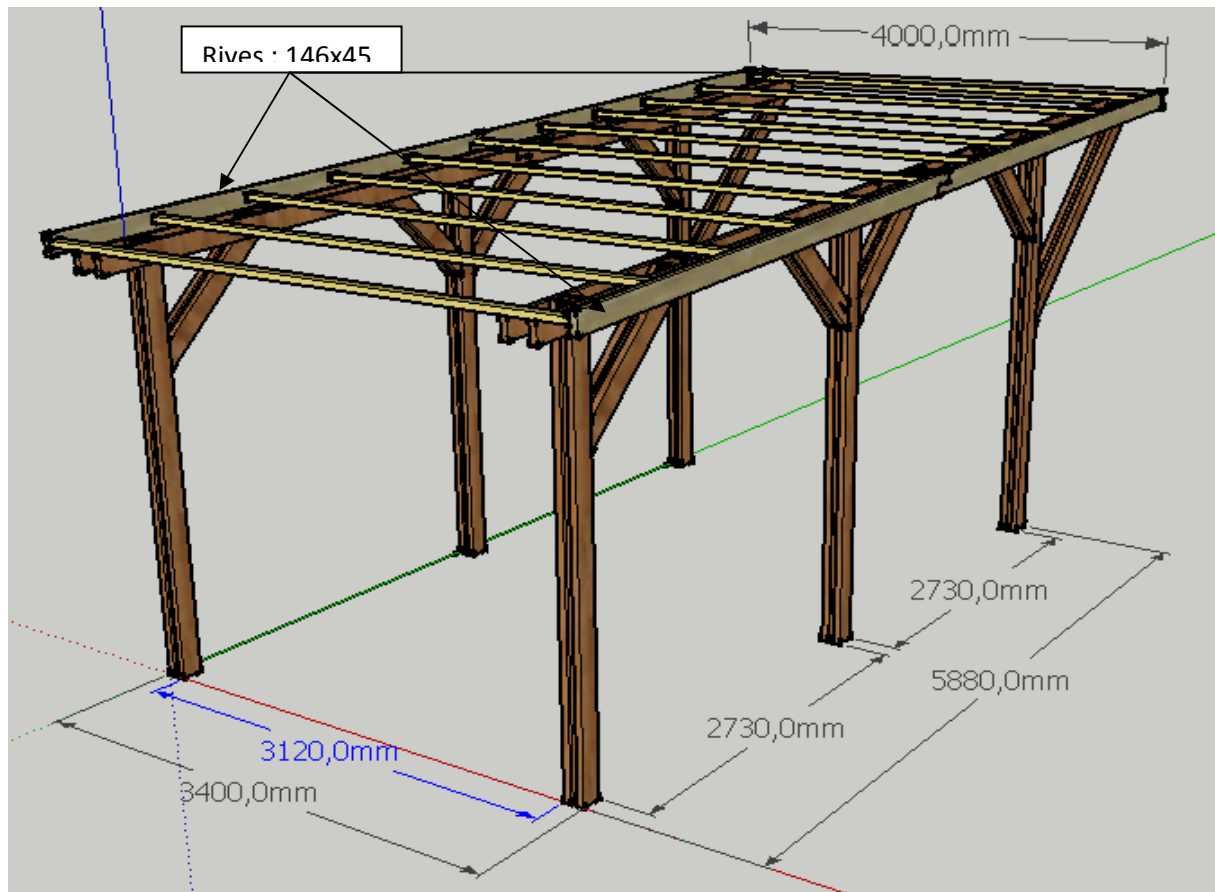
Figure 5: pose des rives
