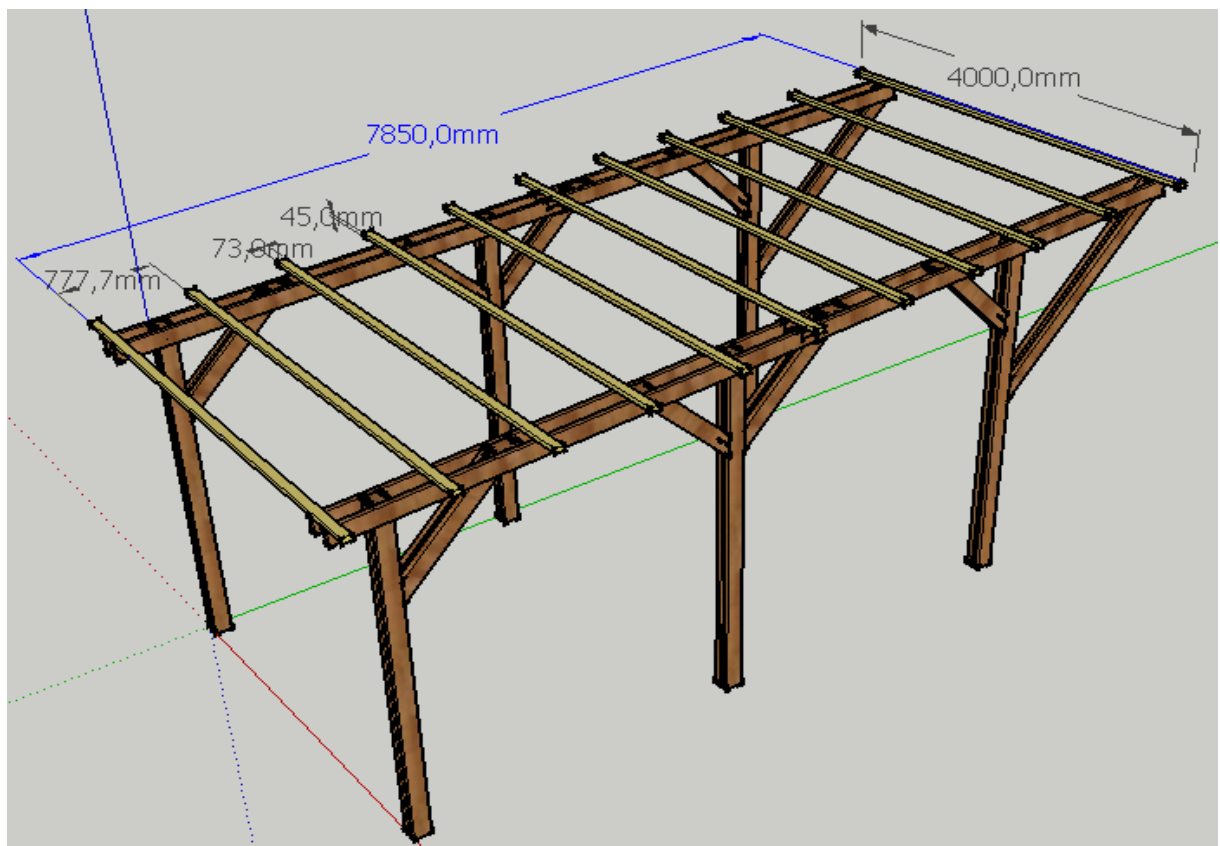
Figure 4: pose des chevrons
